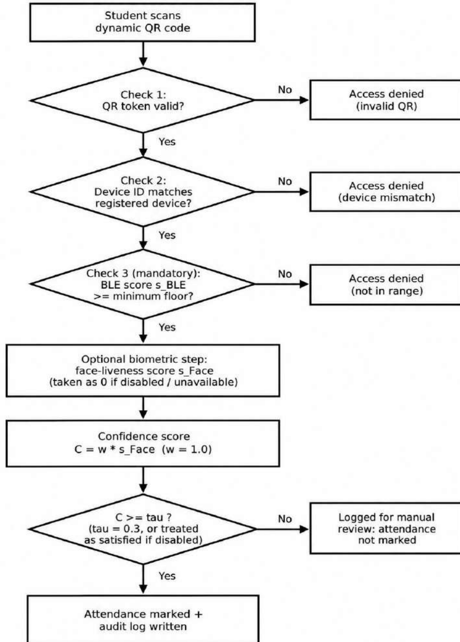
Figure 3: Attendance Verification Sequence
