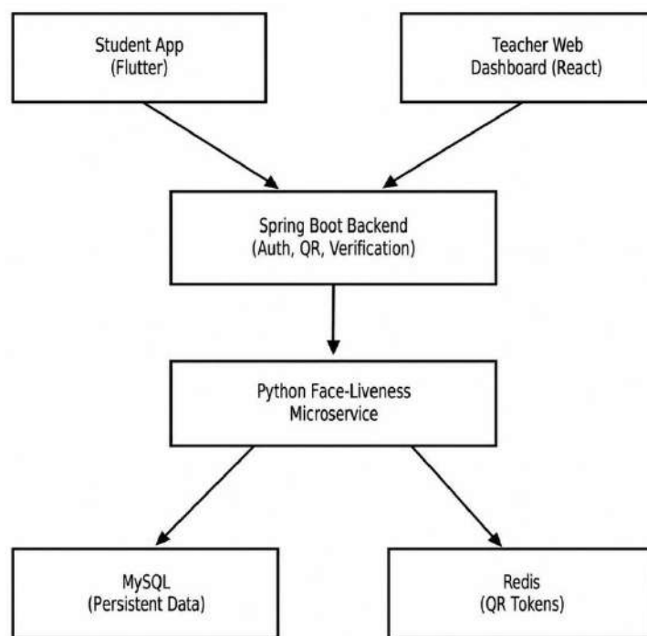
Figure 2: High-Level System Architecture
