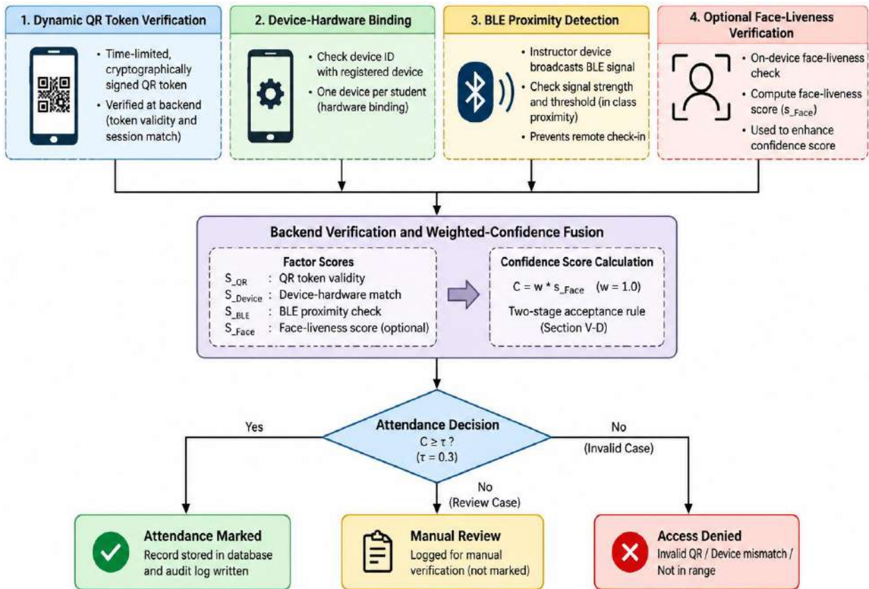
Figure 1: Proposed Multi-Factor Zero-Trust Attendance Verification Framework
